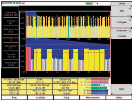
The Code Domain Power (CDP) screen shows 256 or 512 OVSF codes with flexible zoom capabilities.
