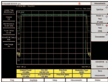
Option 40 displays the first detected timeslot mask as specified in 3GPP TS 05.05.
